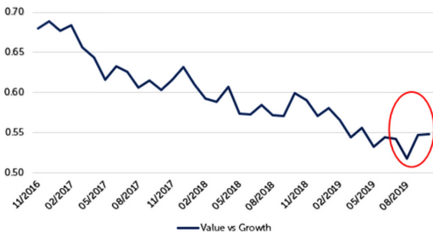
S&P: Value vs Growth
